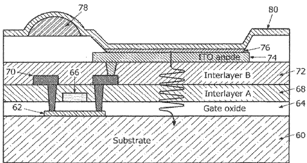
FIG. 6 PRIOR - ART
