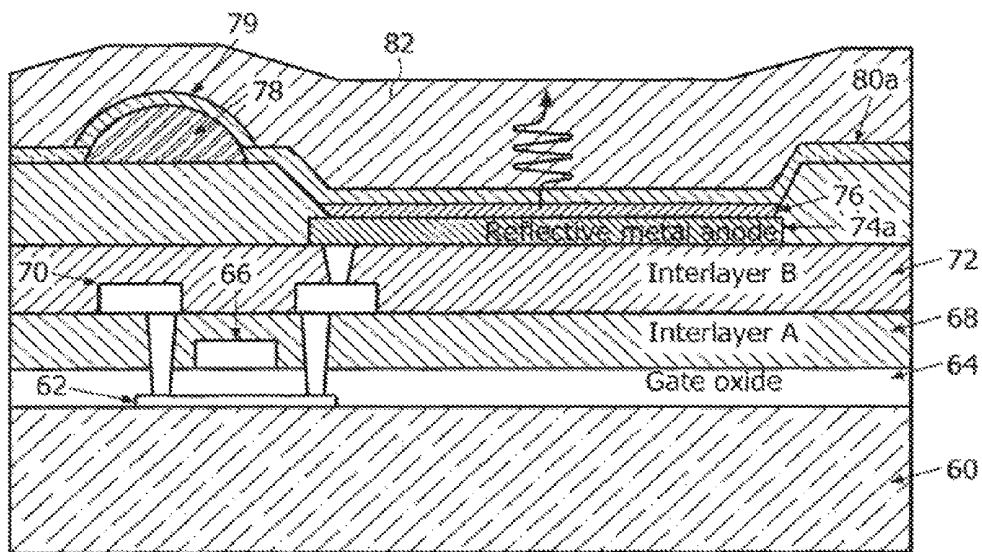
FIG. 7 PRIOR - ART
