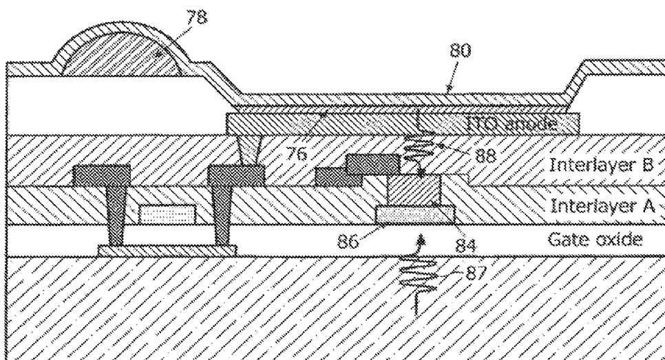
FIG. 8 PRIOR - ART
